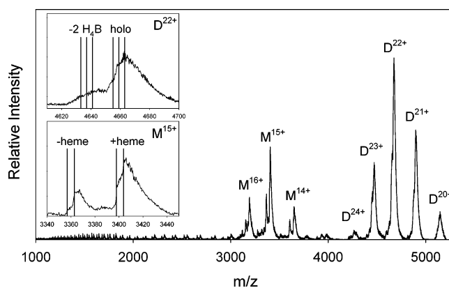
FIGURE 2: ESI mass spectrum of iNOS COD obtained under native conditions [10 mM ammonium acetate (pH 7.5)]. The peaks are identified as monomer (M) or dimer (D) ions with the charge state indicated. (Top inset) Close-up view of the +22 dimer signal. The triplet of lines labeled holo corresponds to the masses expected for dimers representing the light–light, light–heavy, and heavy–heavy monomer combinations (see the legend of Figure 1). These expected dimer masses assume the presence of two heme groups, and two molecules of H 4 B. The triplet on the left indicates the masses expected for dimers after loss of the two H 4 B moieties. (Bottom inset) Close-up view of the +15 monomer peak. The line doublets labeled +heme and –heme correspond to the masses of the two monomer types with and without heme, respectively, in the absence of H 4 B.
