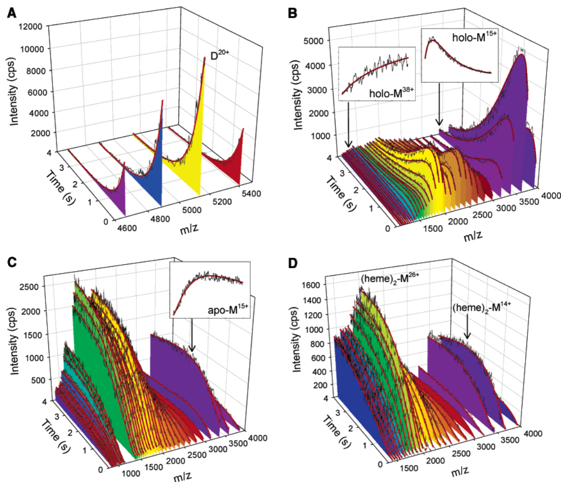
FIGURE 4: Intensity–time profiles for the ionic species that are observed during the acid-induced unfolding of iNOS COD : (A) iNOS COD dimer, (B) heme-bound monomer, (C) apo monomer, and (D) monomer carrying two heme groups. Experimental data are displayed as black lines; dark red curves with colored drop planes are multiexponential fits obtained by global analysis. Selected profiles in panels B and C are displayed separately to highlight the kinetic behavior of the underlying solution-phase species. The gap in panel C is due to the overlap of apo monomers and two-heme monomers, which prevents a kinetic analysis of the corresponding ions in the range around m/z 1400. The data were obtained by operating the rapid-mixing setup in “kinetic mode” (28), i.e., by continuously monitoring ion intensities across the entire m/z range, while continuously increasing the distance between the mixer and ESI source.
